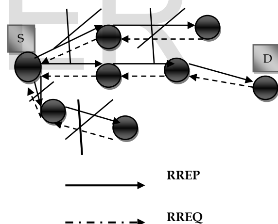
Fig. 1 AODV RREQ and RREP Procedure
